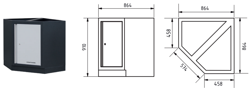
Art. 3964-16 Corner cabinet with 1 door, 1 shelf included
