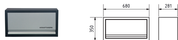
Art. 3964-01 Wall cabinet with gas spring
