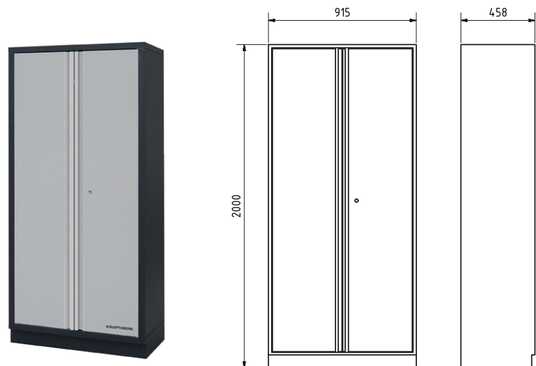
Art. 3964-12 2 doors locker, 4 shelves included
