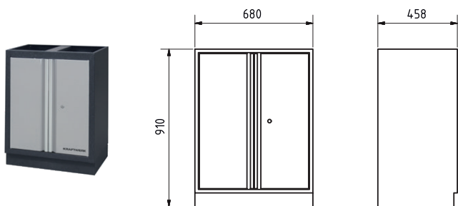
Art. 3964-03 2 doors base cabinet, 1 shelf included
