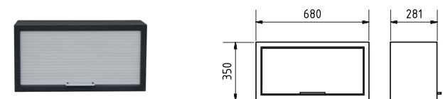
Art. 3964-19 Wall cabinet with roller shutter
