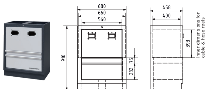
Art. 3964-28 Base cabinet for cable and hose reels with 2 drawers
