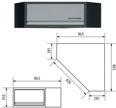
Art. 3964-25 Corner wall cabinet with gas spring
