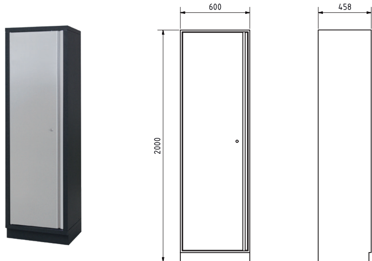
Art. 3964-02 Locker, 4 shelves included
