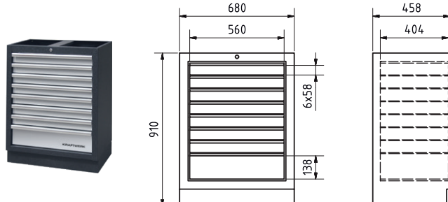
Art. 3964-14 Base cabinet with 8 drawers
