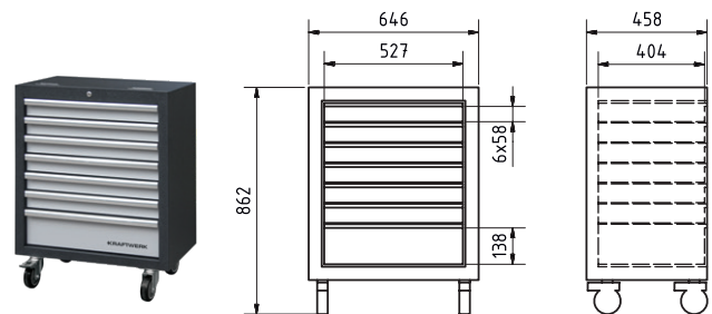
Art. 3964-15 Rolling base cabinet with 7 drawers
