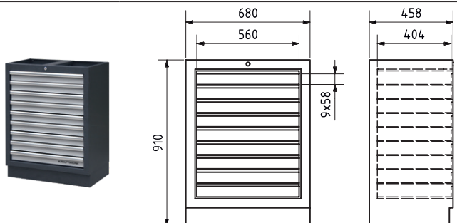
Art. 3964-13 Base cabinet with 9 drawers
