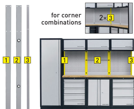
Art. 3964-24 Connect support for 2 elements + 65 x 30 x 1420 mm
