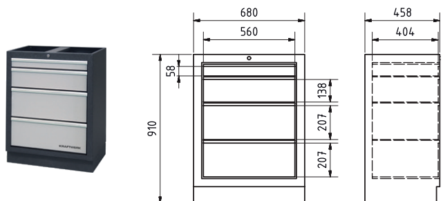
Art. 3964-04 Base cabinet with 4 drawers
