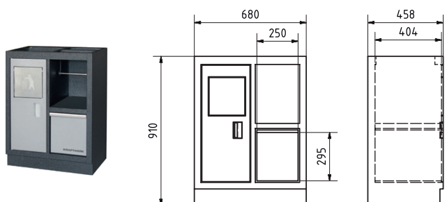
Art. 3964-11 Base cabinet with waste bin and holder for kitchen rolls
