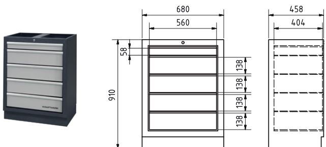
Art. 3964-05 Base cabinet with 5 drawers
